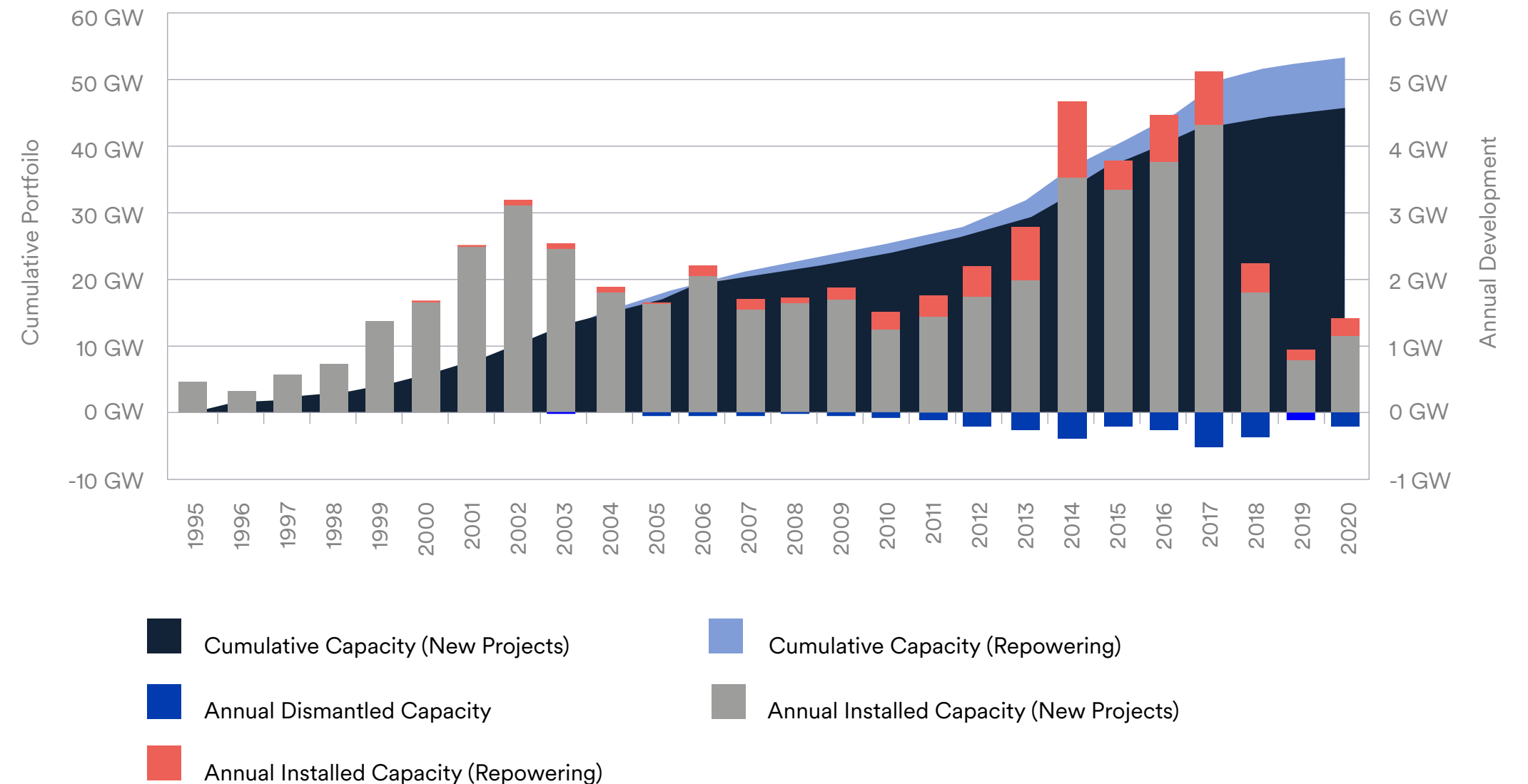
Figure 10: Development of Germany's onshore wind power capacity
